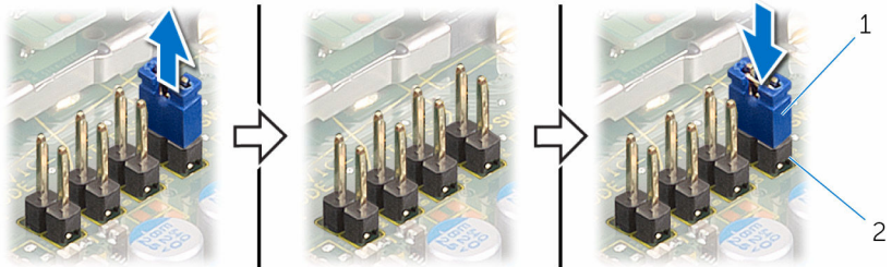
1 jumperplug
